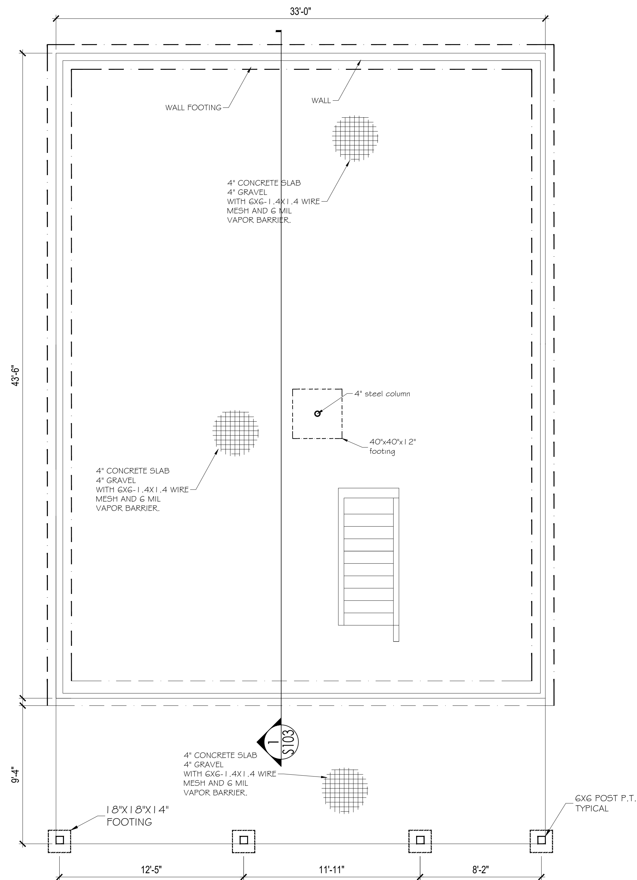
1 FOUNDATION PLAN S101 SCALE: 1/4" = 1'-0"
