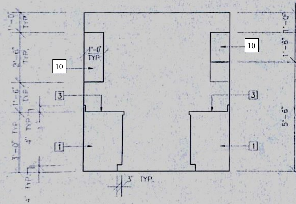
2 TYPICAL KITCHEN (1 BEDROOM) A1/A16 SCALE: 1/2" = 1'-0" (BLDGS. A,B,C,D)
