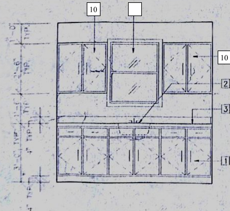
1 TYPICAL KITCHEN (1 BEDROOM) A1/A16 SCALE: 1/2" = 1'-0" (BLDGS. A,B,C,D)
