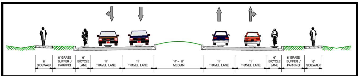
Typical Section of Ager Road
