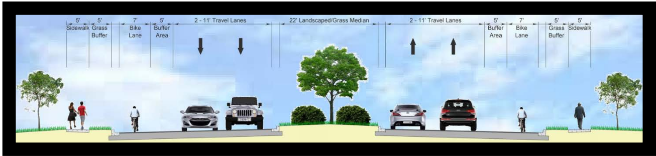
Proposed Typical Section of Lottsford Rd.
