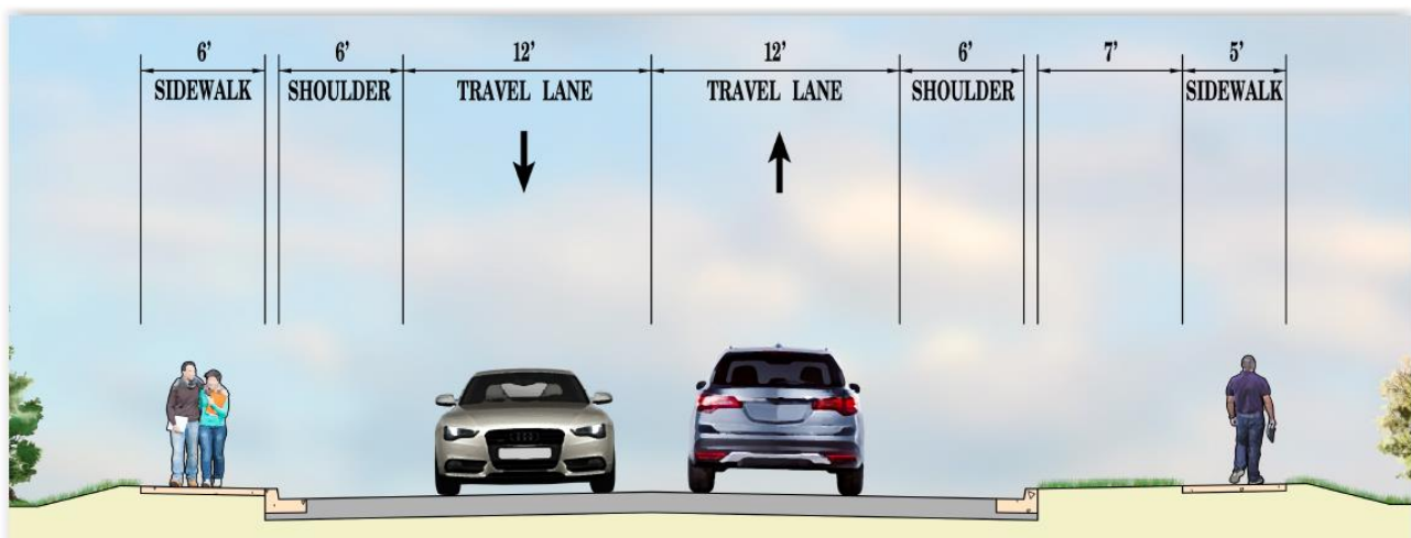
Typical Section of Stuart Lane
