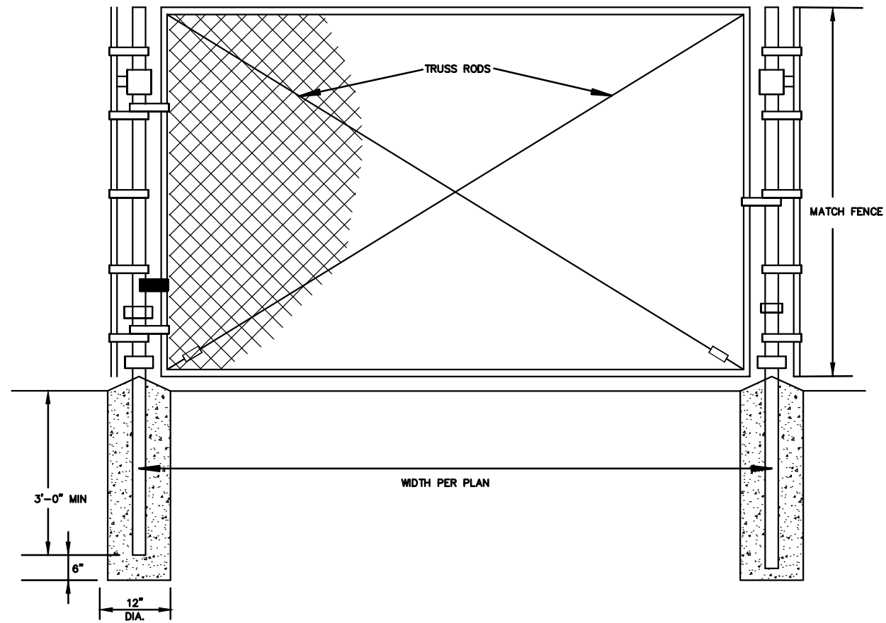
FENCE GATE DETAIL NOT TO SCALE
